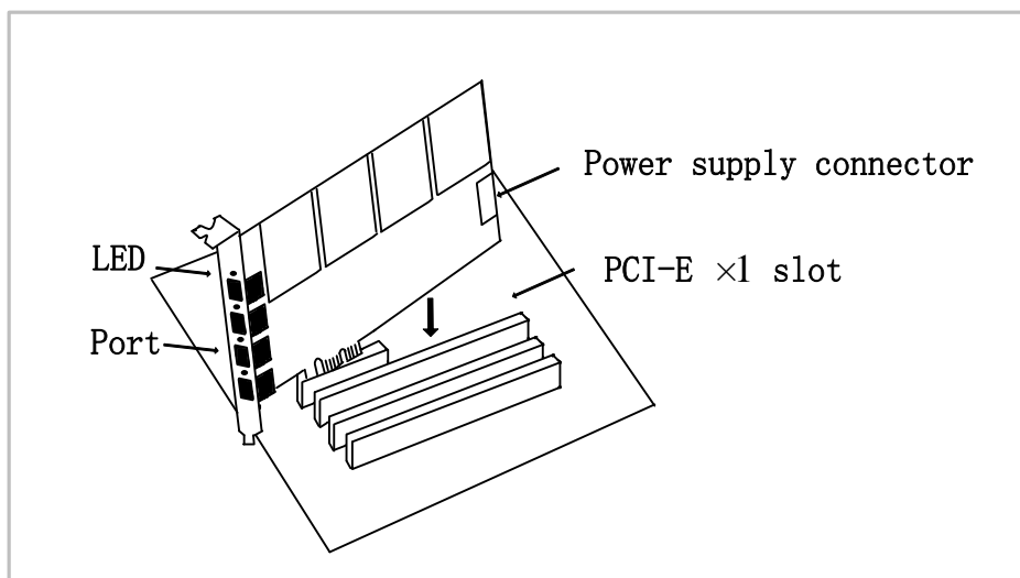
Figure 4 Hardware setup
