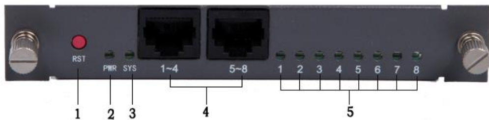
Figure 1-3-2 Front Panel
